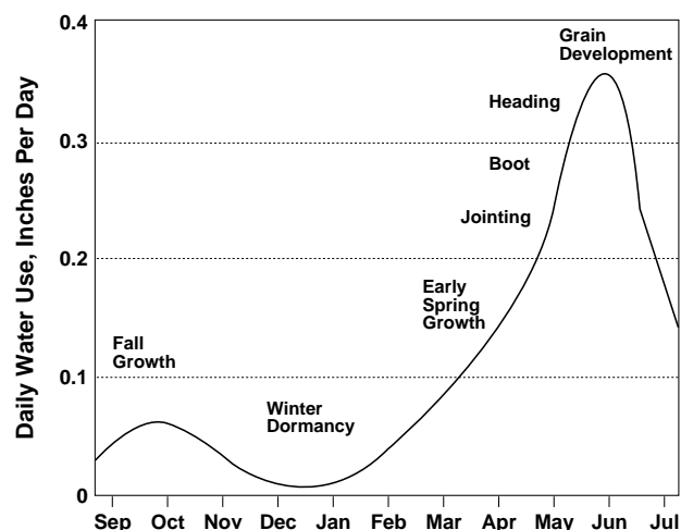
Figure 6. Characteristic water use of winter wheat
